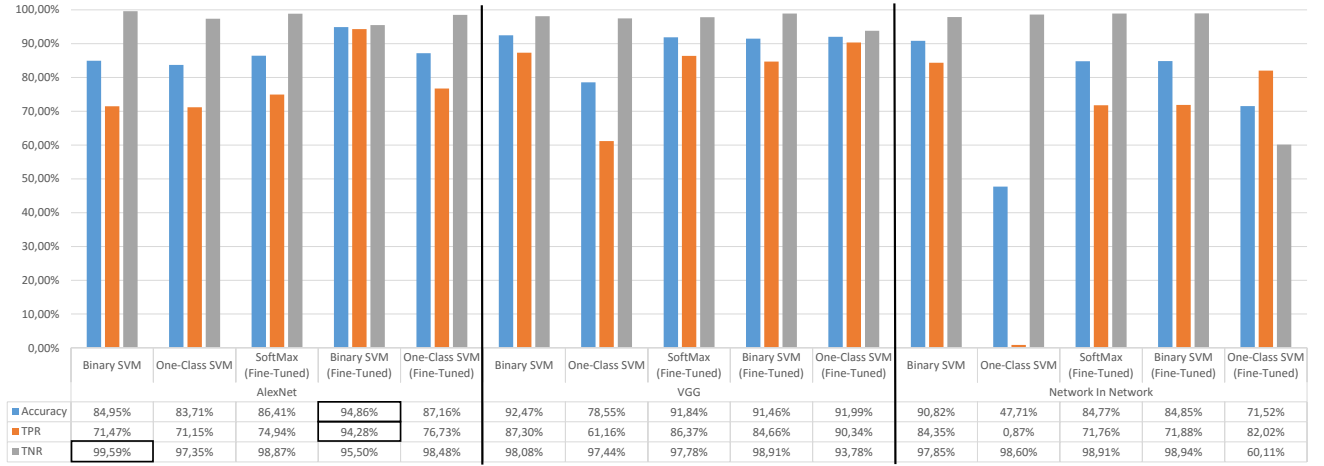
Figure 2: Results of the experiments. Values indicating best performances are boxed . Left: results related to the AlexNet model. Middle: results related to the VGG model. Right: results related to the Network In Network model.
