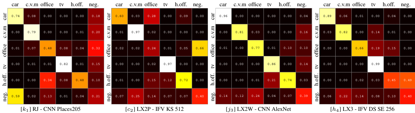
Figure 5. Confusion matrices of the four the best performing methods on the considered devices. Columns represent the ground truth classes, while rows represent the predicted labels. The original confusion matrices have been row-normalized (i.e., each value has been divided by the sum of all the values in the same row) so that each element on the diagonal represents the per-class True Positive Rate. Each matrix is related to the row of Table 2 specified by the identifier in brackets. The following abbreviations are used: c.v.m - coffee vending machine, h.off - home office, neg. - negatives.
