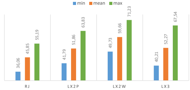
Figure 4. Minimum, average and maximum accuracies per device. As can be noted, all the statistics are higher for the LX2W-related experiments. This suggests that the task of recognizing personal contexts is easier for images acquired using such device.
