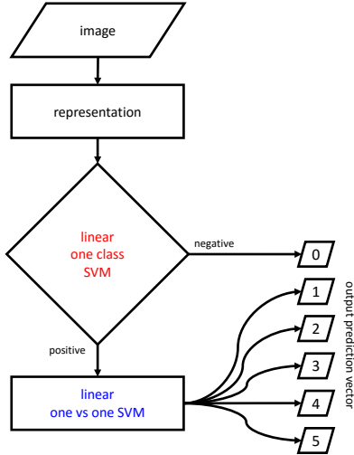
Figure 3. Diagram of the proposed classification pipeline.
